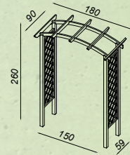
Rose Arch 40121
