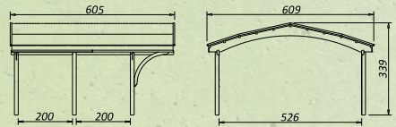
Nevada Double Carport Panels shown are not included 41835 609 x 605 x 339
