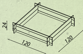
Economy Veggiebed 10870 24 x 120 x 120
