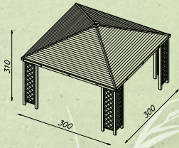
Rimini Pavilion 41500
