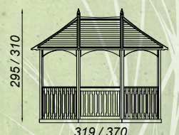
Timber Roof 42121 42122
