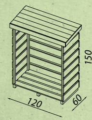
Log Store 50301 150 x 120 x 60
