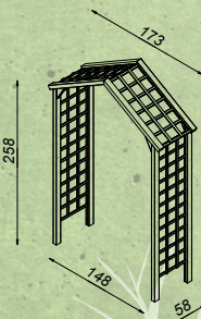
Chester Arch 40193
