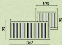
Windsor Fence and Gate 21175 90 x 100 21171 90 x 180
