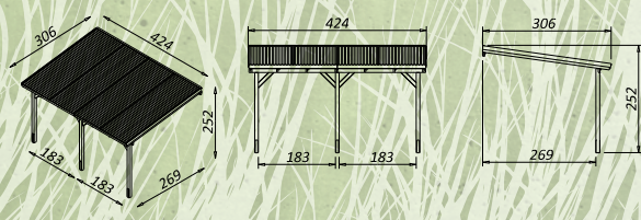
Contego Lean-to-Carport 41847 306 x 424 41848 306 x 514 41849 306 x 704
