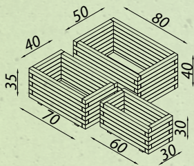
Royal Rectangular Planter 50405 30 x 60 x 30 50461 35 x 70 x 40 50462 40 x 80 x 50
