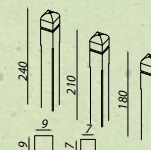
Fence Post - Lux Diamond Top 14117 180 x 7 x 7 14118 210 x 7 x 7 14125 240 x 7 x 7 14128 240 x 9 x 9
