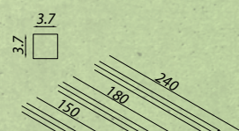
Tree Stake (Post) 14181 150 x 3.7 14182 180 x 3.7 14183 240 x 3.7
