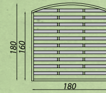
Malvern Gate 21434
