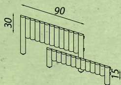
Border Section 10850 15 x 90 10852 30 x 90
