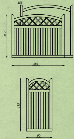
Dallas Convex Fence and Gate 21115 90 x 183 21114 150 x 183 21113 183 x 183
