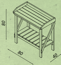
Potting Bench 52034 80 x 40 x 80
