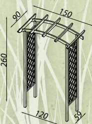
Arcade Light 40146
