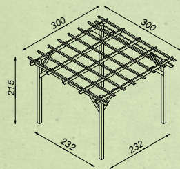
Henley Pergola 41853
