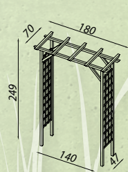
Mendip Arch 41021
