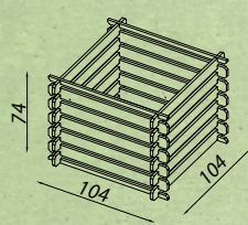
Garden Composter 52001 74 x 104 x 104
