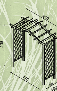
Dover Arch 40194
